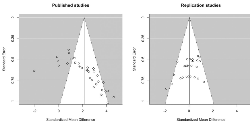
Figure 1. Funnel plots including published studies (left panel) and our own replication studies (right panel) in which MDZ was used as amnesic agent. Each point represents an observed effect size Hedges’ g against its SE. Visual inspection of the plot on the right panel shows that our replication studies are symmetrically scattered around the effect estimate of 0.04, indicating that the estimated effect size is close to zero and suggesting that no trend in one particular direction was observed across studies. In contrast, the plot of published studies (left panel) clearly shows asymmetry, and the reported effect sizes seem to depend strongly on the research group in which the studies were performed (represented by the different symbols in the left plot). Egger’s test confirmed plot asymmetry ( p < 0.0001 ), even when considering the moderating influence of research group. One should be careful to attach value to the estimated effect size shown in the left funnel plot, given the evidence for publication bias and because the nesting of studies within research groups is not accounted for. The funnel plots were based on the meta-analytic models without moderators. Symbols represent the research group in which each study was performed (left panel) or the lab space that was used (right panel). Note that three of our exact replication studies (right panel) were performed in the same lab space as some of the original, published studies (left panel).
