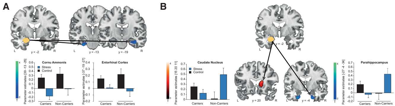
Figure 5. Stress and MR haplotype effects on brain connectivity in Experiment II. A , Stress resulted in decreased amygdala-hippocampus connectivity (cornu ammonis: p_{FWE} = 0.043 , entorhinal cortex: p_{FWE} = 0.061 ). MR haplotype carriers showed reduced amygdala-anterior parahippocampus connectivity under stress (both p_{FWE} \leq 0.063 ; B ), whereas under control conditions, MR haplotype carriers showed increased amygdala-caudate nucleus coupling ( p_{FWE} = 0.018 ; C ). Activations are superimposed on coronal sections of a T1-weighted template image and represented in red when greater blue when reduced in MR haplotype carriers, the anatomic mask is indicated in yellow. L corresponds to the left, R to the right side of the brain, and error bars represent SEM.
